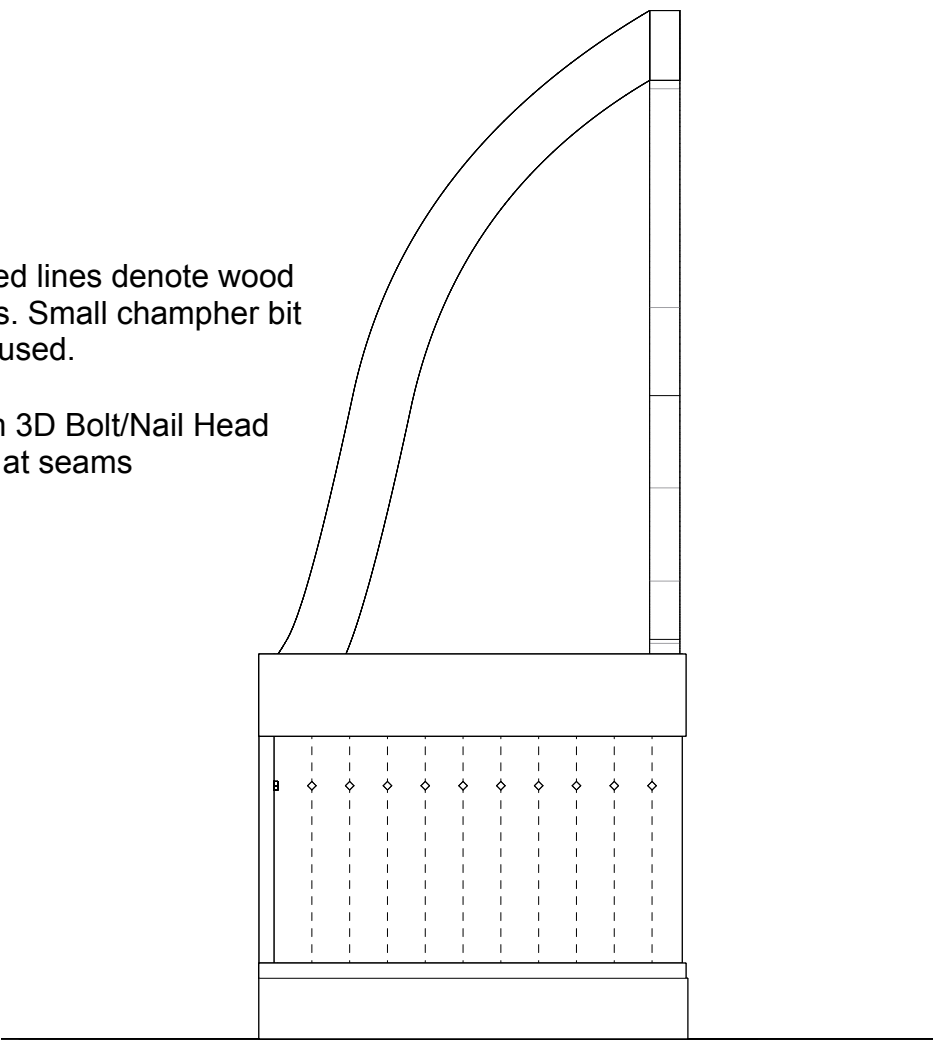
03 Bedrom Side (External) Scale 1:25
