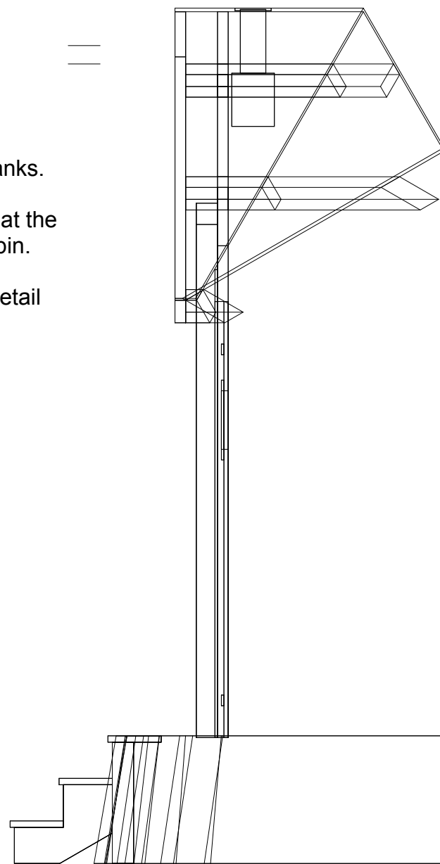
03 Oaken Sauna View 2 Scale 1:25
