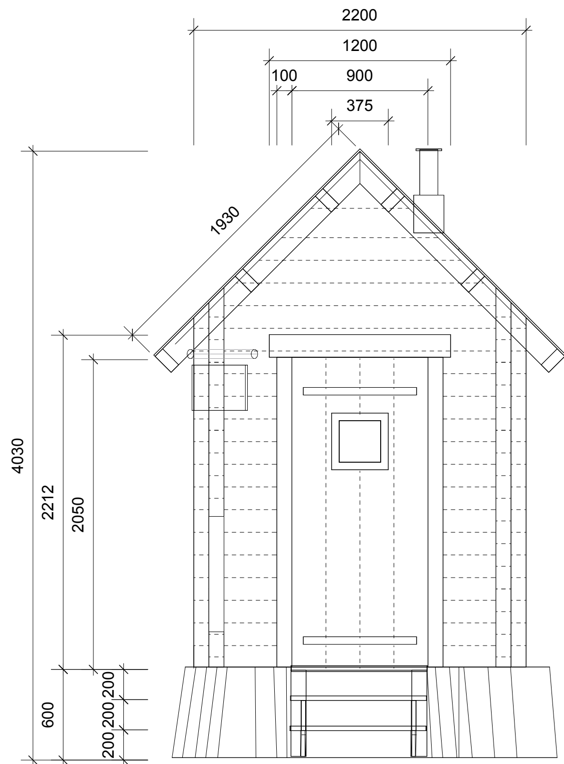
02 Oaken Sauna View 1 Scale 1:25
