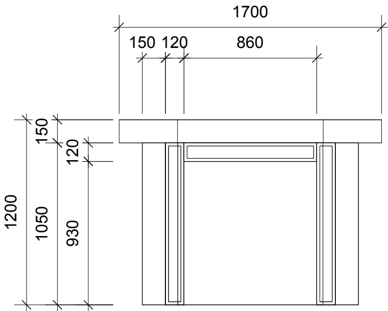
01 Fireplace Front Scale 1:25
