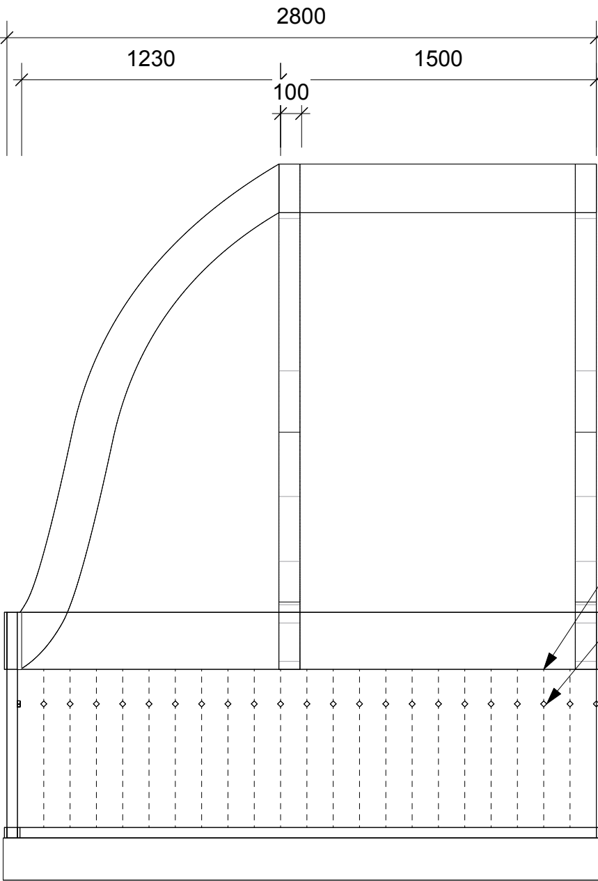
01 Bedrom Front Scale 1:25
