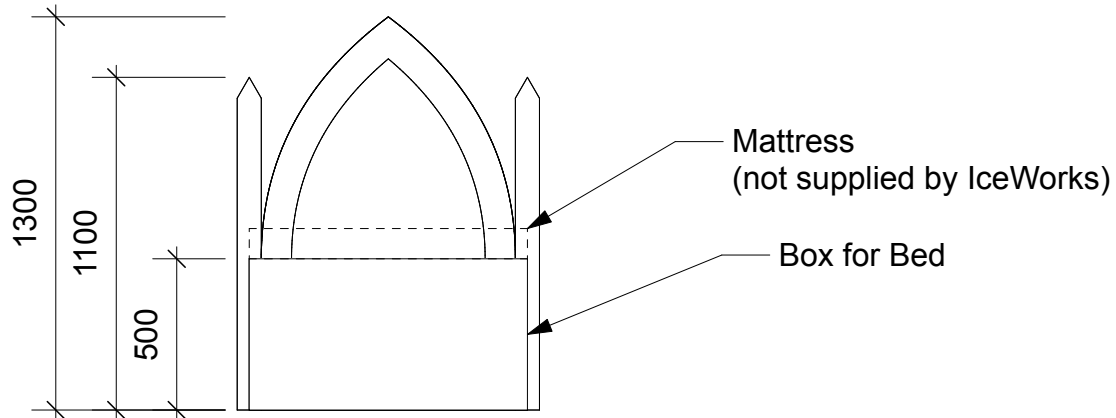
02 Bed Side Scale 1:25
