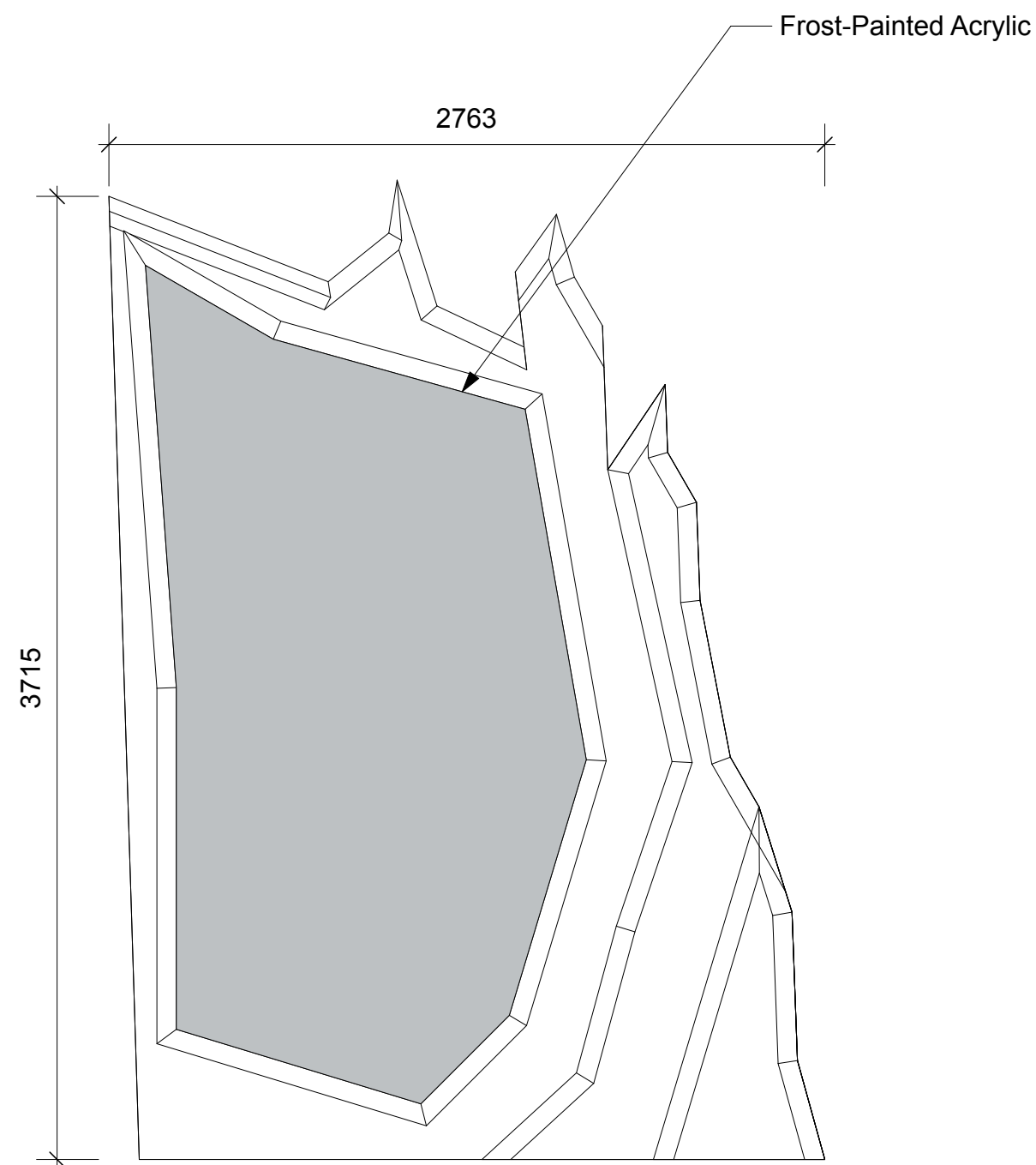
09 Ice Palace PS Front Scale 1:25
